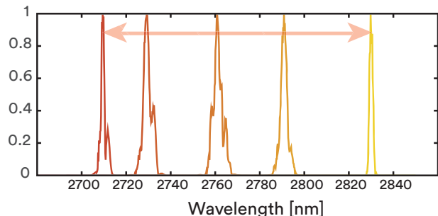
Typical spectrum 3
