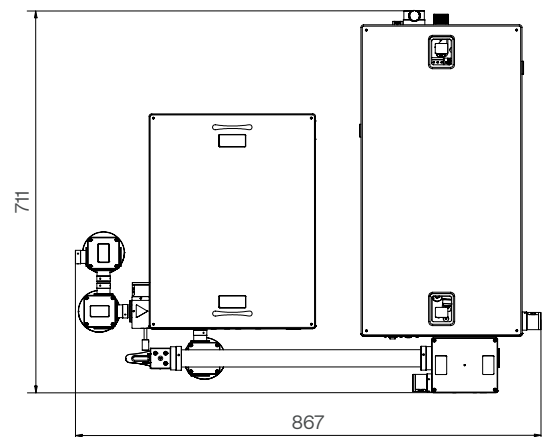
ORPHEUS-PS with SHBC drawing
